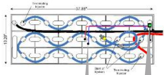
SmartBlinky™ shown on 18-100-11 Instant Install™ Layout
